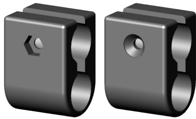
SR2XR20K/M6(M8)
