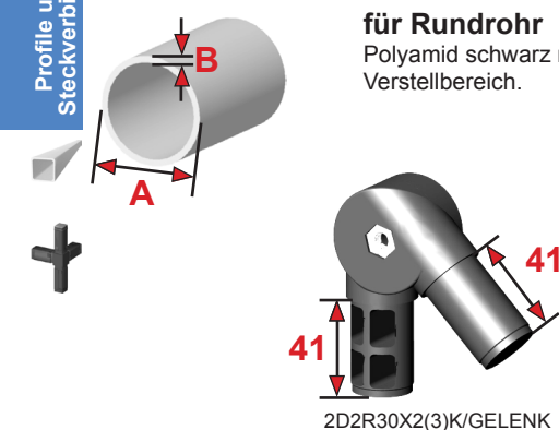
2D2R30X2(3)K/GELENK
